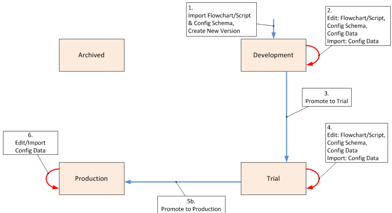
Figure 17 Transitions from Development to Production State
